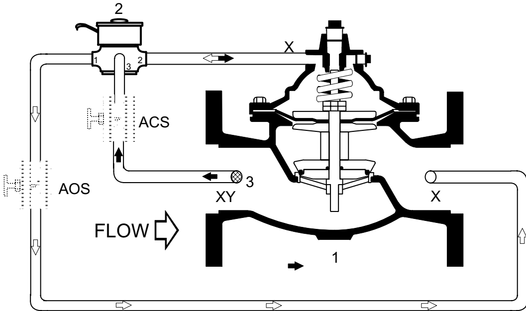
Flow Direction Shown: Under the Seat Optional 'R' Flow Over the Seat: 113-12R/6113-12R
